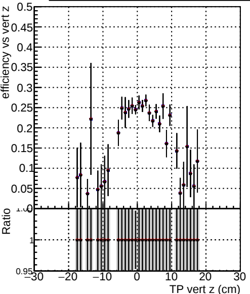
Efficiency vs TP vert z (cm) Legend: DQM_TT_original_time DQM_TT_newscoreonlyINIT_time DQM_TT_modified_time
