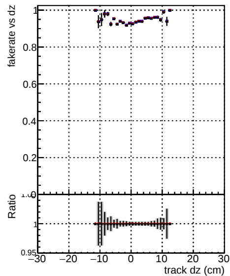
Fake rate vs dz Legend: DOM TT original time newscoronly/INIT_time DOM TT modified time
