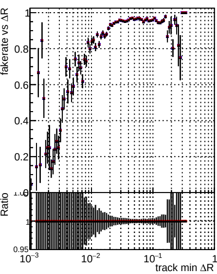
Fake rate vs \Delta R (track, jet) Legend: DQM TT original_time DQM TT newscoreonlyINIT_time DQM TT modified_time
