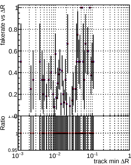
Fake rate vs ΔR(track, jet) Legend: DOM TT original_time DOM TT newscoreonlyINIT_time DOM TT modified_time
