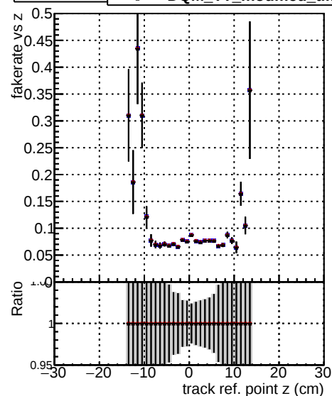
Fake rate vs verpos Legend: \bullet DQM TT original_time \bullet DQM TT newscoreonlyINIT_time \bullet DQM TT modified_time
