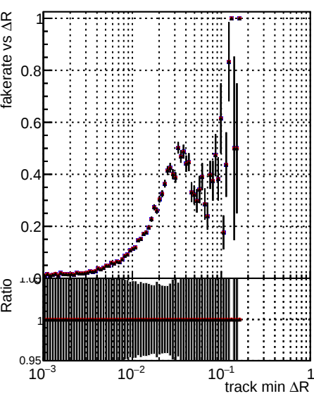
Fake rate vs \Delta R(\text{track, jet}) Legend: \text{DQM\_TT\_original\_time} (black line) \text{DQM\_TT\_newscoreonlyINIT\_time} (red line) \text{DQM\_TT\_modified\_time} (black line)
