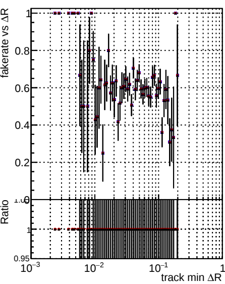
Fake rate vs \Delta R(\text{track, jet}) Legend: DQM TT original_time DQM TT newscoreonlyINIT_time DQM TT modified_time
