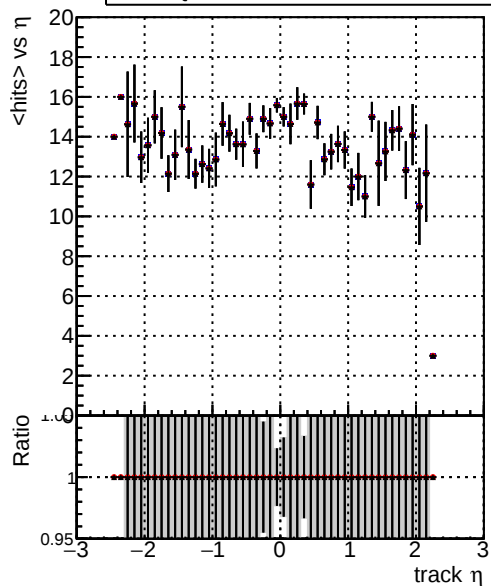
mean hits — DQM_TT_original_time — DQM_TT_newscoreonlyINIT_time — DQM_TT_modified_time
