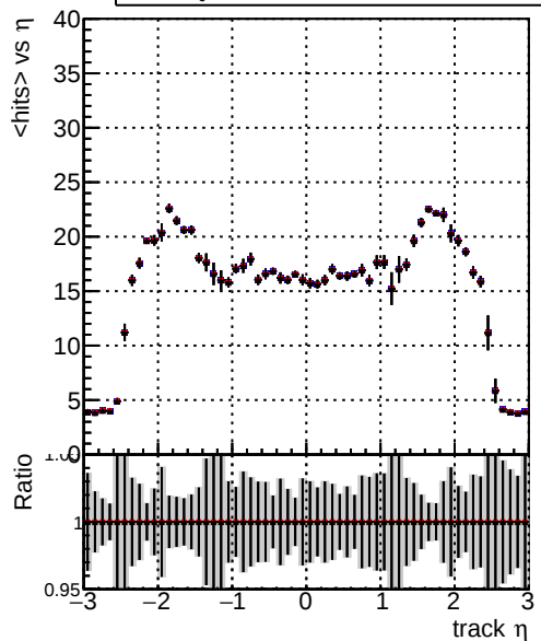
mean hits — DQM_TT_original_time — DQM_TT_newscoreonlyINIT_time — DQM_TT_modified_time
