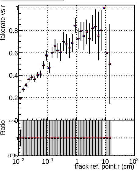
Fake rate vs v DOM TT original_time DOM TT newscoreonlyINIT_time DOM TT modified_time
