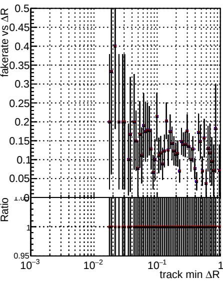
Fake rate vs \Delta R(\text{track, jet}) Legend: DOM TT original_time DOM TT newscoreonlyINIT_time DOM TT modified_time
