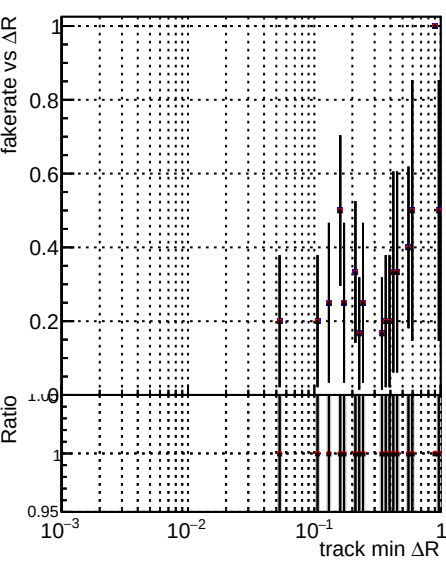
Fake rate vs ΔR(track, jet) Legend: DQM_TT_original_time DQM_TT_newscoreonly DQM_TT_modified_time
