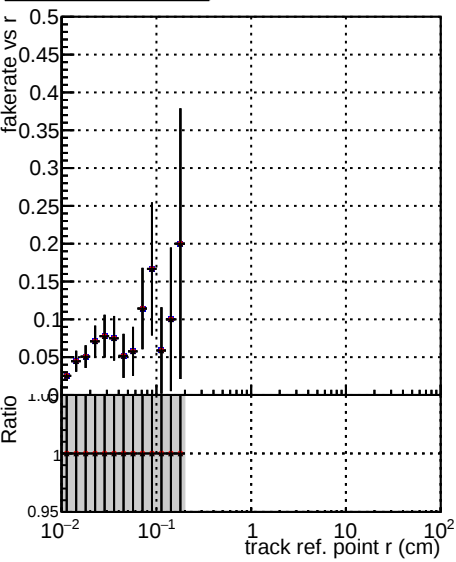
Fake rate vs verpos Legend: - DQM TT original_time (blue) - DQM TT newscoreonly (red) - DQM TT modified_time (black)
