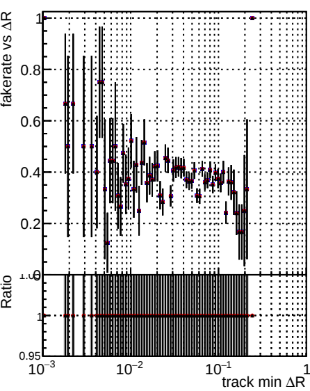
Fake rate vs \Delta R(\text{track, jet}) Legend: DQM TT original_time (blue circle) DQM TT newscoreonly (red circle) DQM TT modified_time (black circle)
