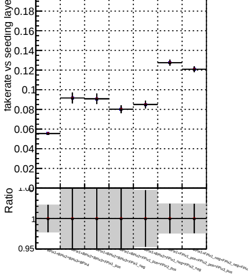
fakrate vs seeding layers
