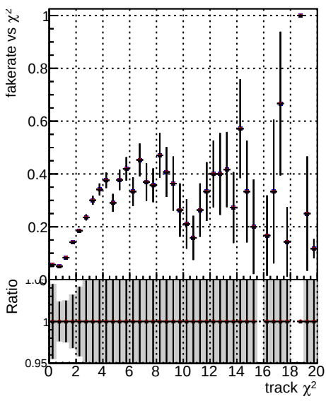
Fake rate vs. DOM TT original time DOM TT newscoronlyINIT_time DOM TT modified time
