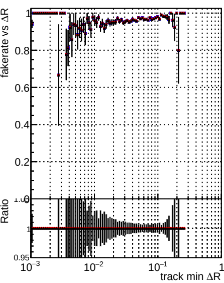
Fake rate vs \Delta R (track, jet) Legend: - DQM TT original_time (black line) - DQM TT newscoreonly (red line) - DQM TT modified_time (blue line)
