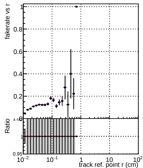
Fake rate vs verpos Legend: —•— DQM TT original_time —•— DQM TT newscoreonlyINIT_time —•— DQM TT modified_time
