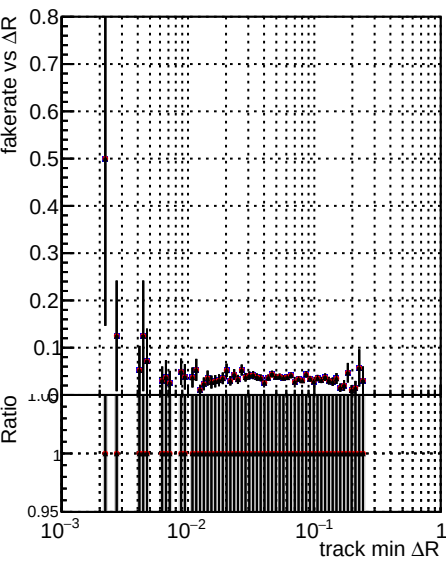
Fake rate vs \Delta R(\text{track}, \text{jet}) Legend: \Delta R(\text{track}, \text{jet}) original_time \Delta R(\text{track}, \text{jet}) newscoreonly \Delta R(\text{track}, \text{jet}) modified_time
