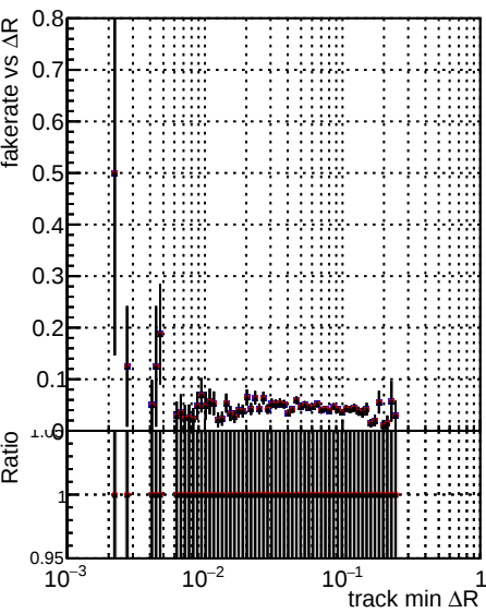
Fake rate vs \Delta R(\text{track}, \text{jet}) Legend: DQM TT original_time DQM TT newscoreonly DQM TT modified_time
