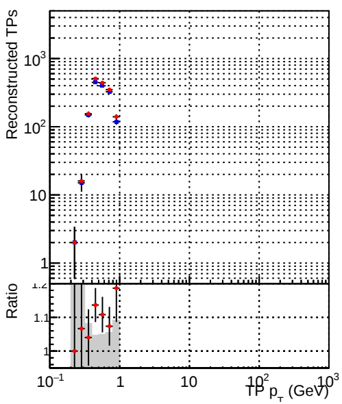
—•— DQM_TT_original —•— DQM_TT_newscoreonlyINIT
