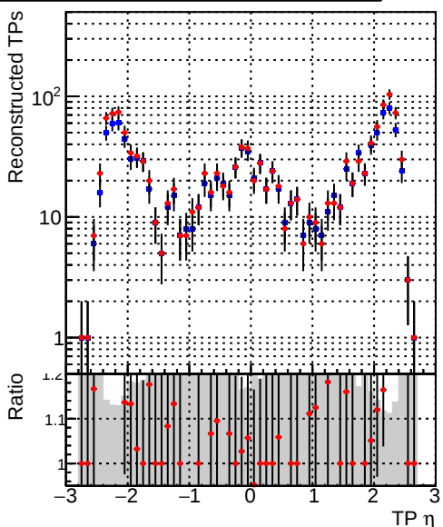
—•— DQM_TT_original —•— DQM_TT_newscoreonlyINIT
