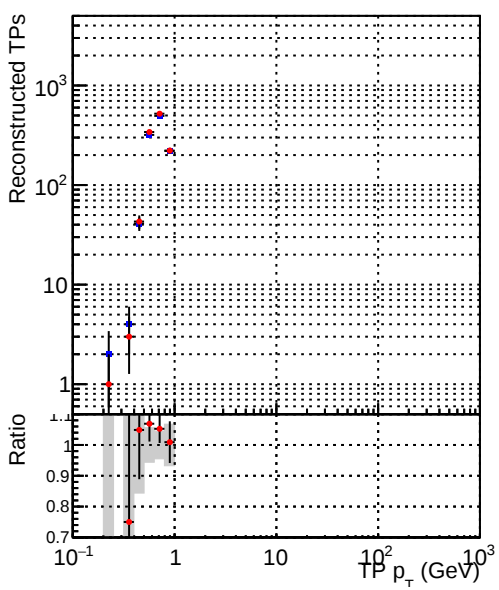
Legend: DQM_TT_original (blue dots), DQM_TT_newscoreonlyINIT (red dots)
