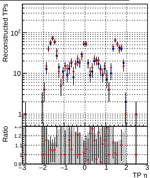
Legend: DQM_TT_original (blue dots), DQM_TT_newscoreonlyINIT (red dots)
