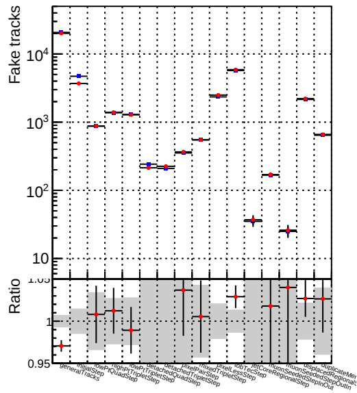
DQM_TT_newscoreonlyINIT
