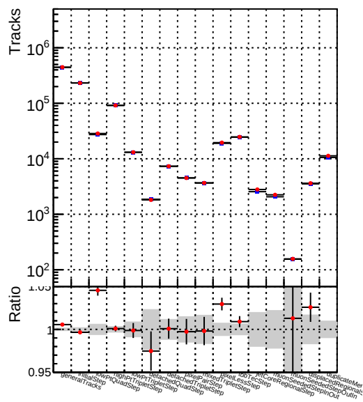
DQM_TT_original
