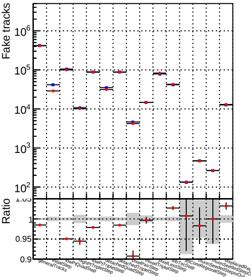
Number —●— DQM_TT_newscoreonlyINIT
