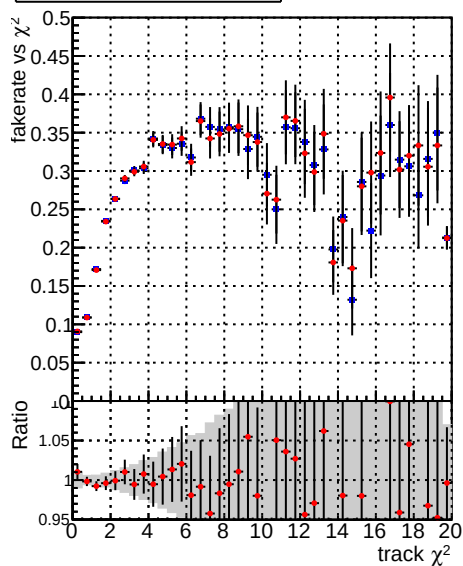
Fake rate vs. —●— DQM TT original —●— DQM TT newscoreonlyINIT
