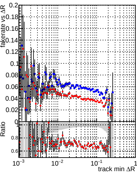
Fake rate vs ΔR(track, jet) DQM_TT_original DQM_TT_newscoreonlyINT
