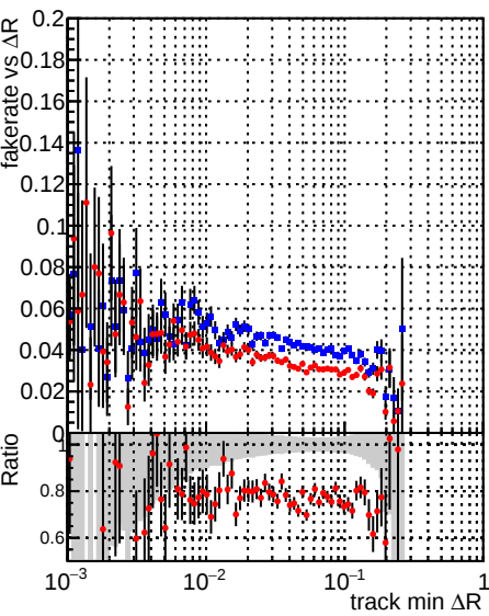
Fake rate vs \Delta R (track, jet) DQM_TT_original DQM_TT_newscoreonlyINIT
