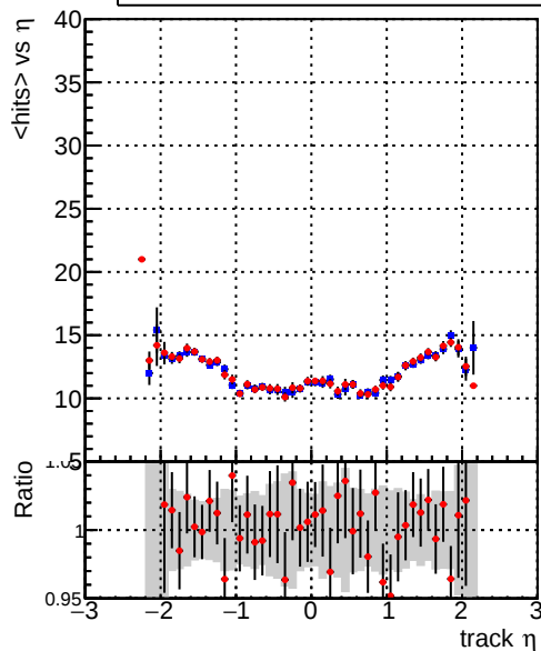
mean hits Legend: — DQM_TT_original, — DQM_TT_newscoreonlyINIT
