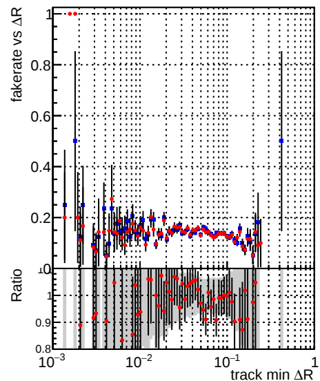
—•— DQM_TT_original —•— DQM_TT_newscoreonlyINIT
