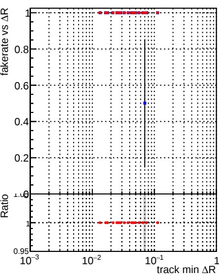
Legend: DQM_TT_original (blue dots with error bars), DQM_TT_newscoreonlyINIT (red dots with error bars)
