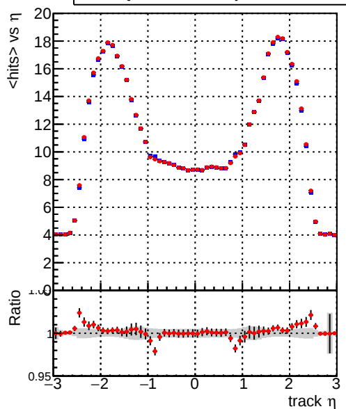
mean hit Legend: DQM_TT_original (blue line), DQM_TT_newscoreonlyINIT (red line)
