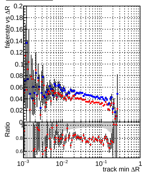
—•— DQM_TT_original —•— DQM_TT_newscoreonlyINT
