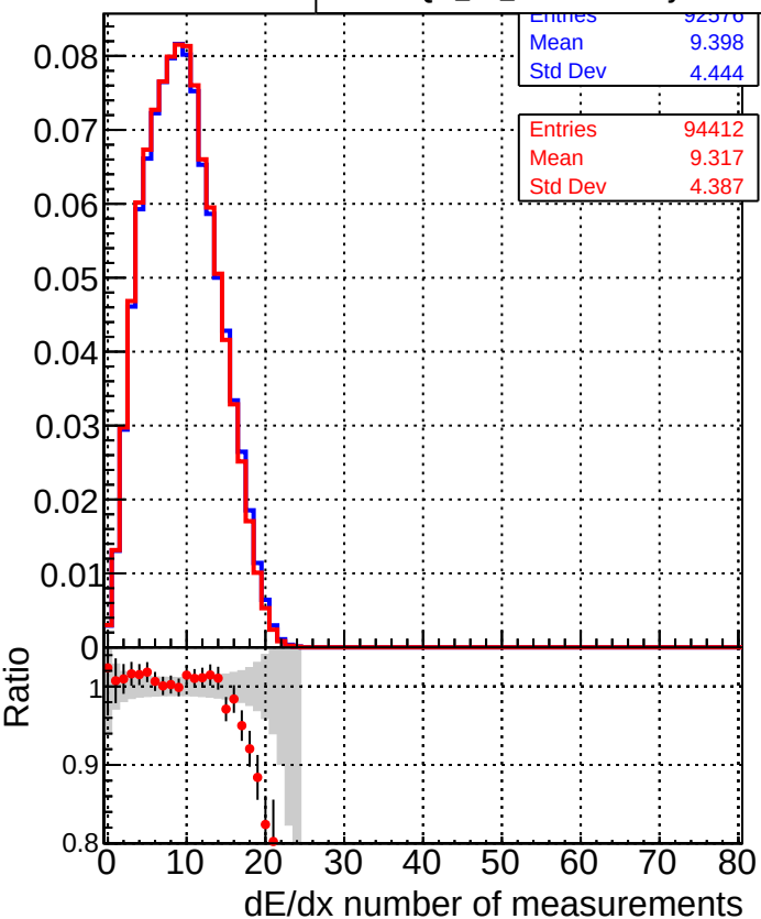
■ DQM_TT_original ● DQM_TT_newscoreonlyINIT
