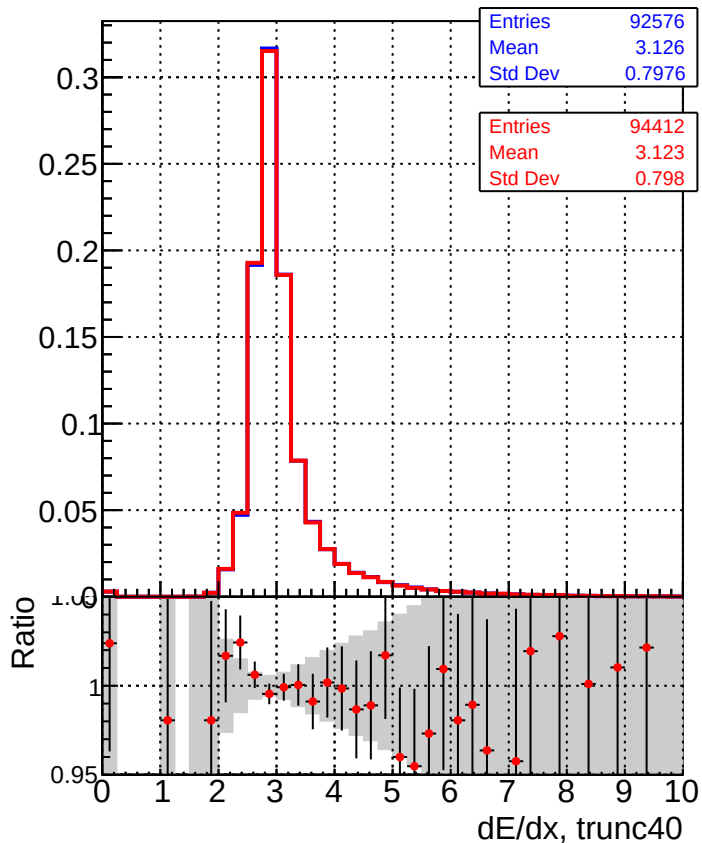
■ DQM_TT_original ● DQM_TT_newscoreonlyINIT
