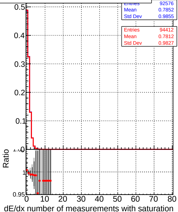
■ DQM_TT_original ● DQM_TT_newscoreonlyINIT
