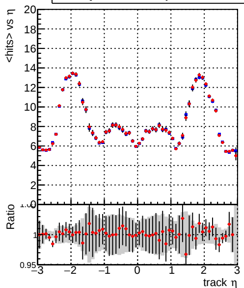
mean hits vs \eta Legend: DQM_TT_original (blue line), DQM_TT_newscoreonlyINIT (red line)
