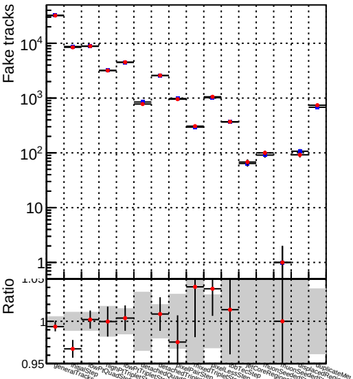
Number —●— DQM_TT_newscoreonlyINIT
