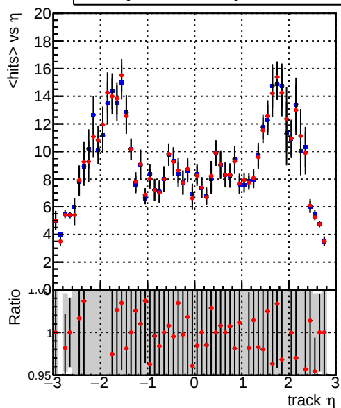
mean hits vs \eta — DQM_TT_original — DQM_TT_newscoreonlyINIT
