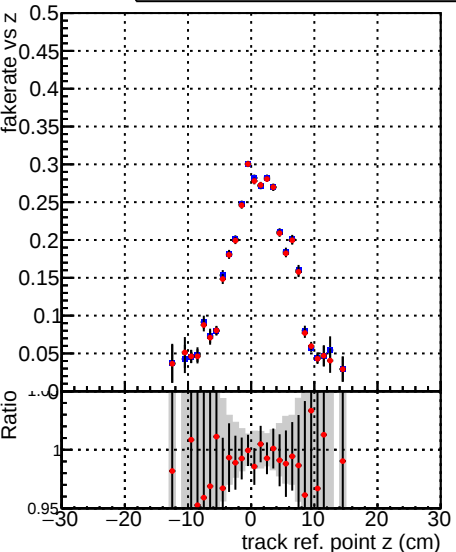
—●— DQM_TT_original —●— DQM_TT_newscoreonlyINT
