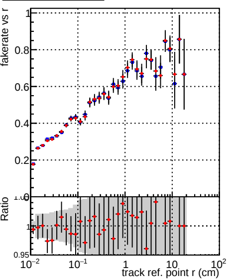
—●— DQM_TT_original —●— DQM_TT_newscoreonlyINT
