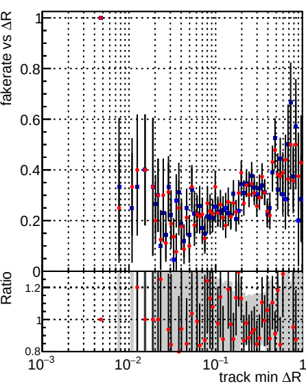
Fake rate vs \Delta R(\text{track, jet}) DQM_TT_original DQM_TT_newscoreonlyINIT
