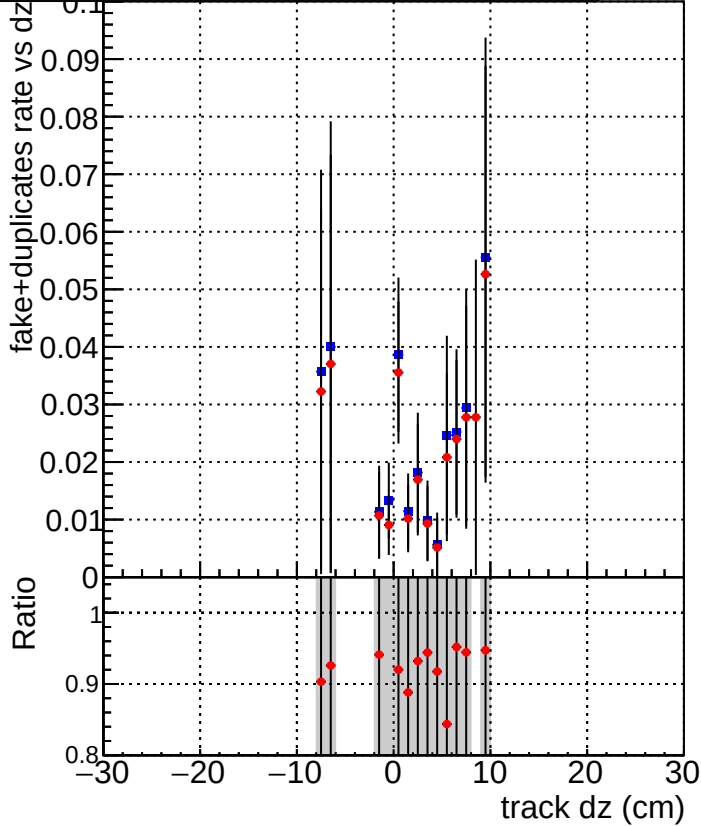
DQM_TT_original DQM_TT_newscoreonlyINIT
