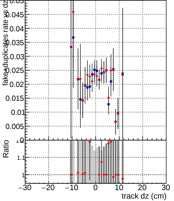
DQM_TT_original DQM_TT_newscoreonlyINIT
