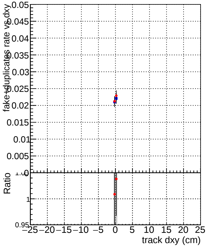
DQM_TT_original DQM_TT_newscoreonlyINIT
