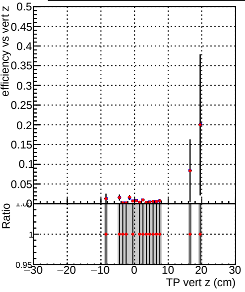
Efficiency vs vert z Legend: DQM_TT_original DQM_TT_newscoreonlyINIT
