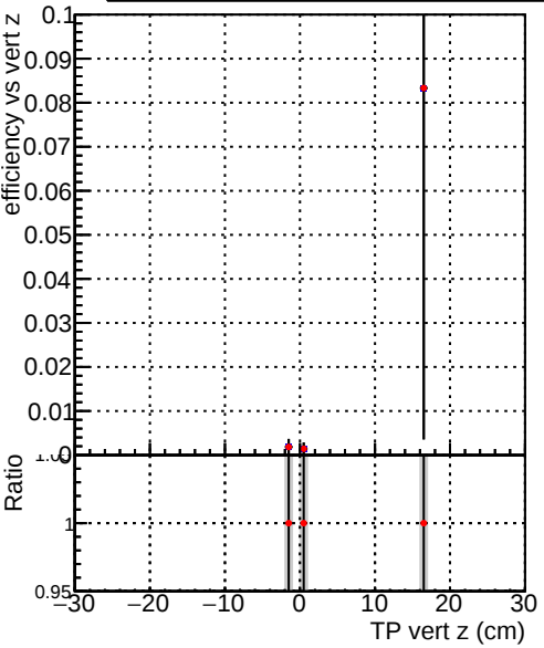
Efficiency vs vertpos Legend: DQM_TT_original (blue line with dots), DQM_TT_newscoreonlyINIT (red line with dots)
