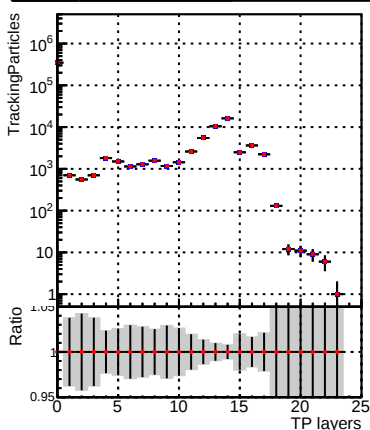
N of sim —●— DQM_TT_newscoreonlyINIT
