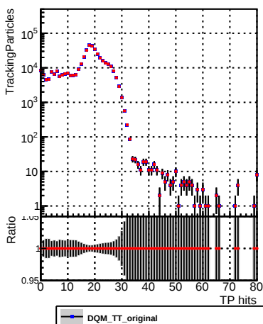
N of sim —●— DQM_TT_newscoreonlyINIT
