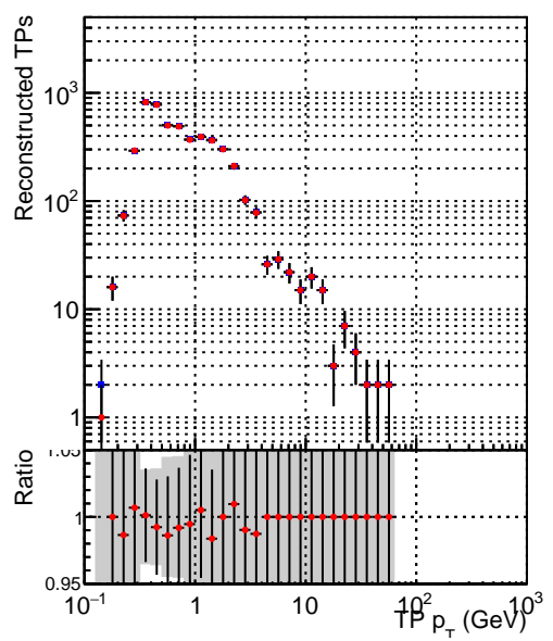
■ DQM_TT_original ● DQM_TT_newscoreonlyINIT
