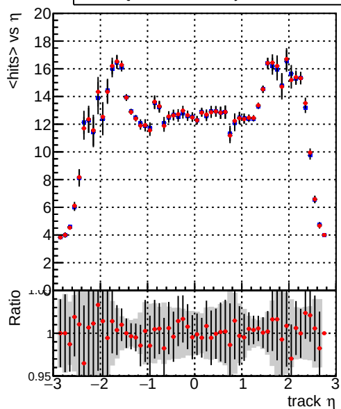
— DQM_TT_original — DQM_TT_newscoreonlyINIT mean hits
