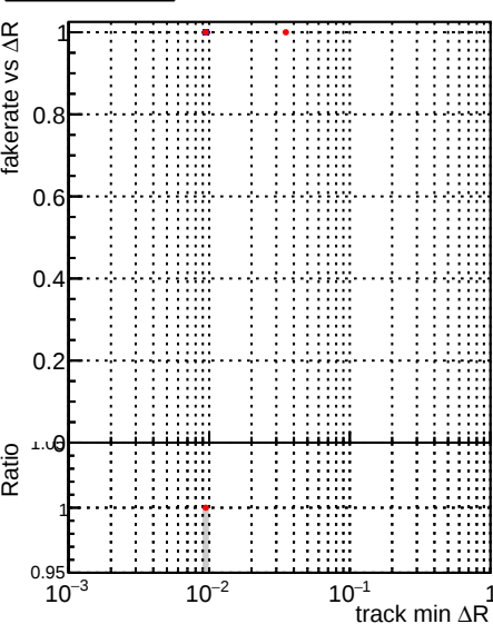
Fake rate vs \Delta R(\text{track, jet}) Legend: \square DQM_TT_original \bullet DQM_TT_newscoreonlyINIT
