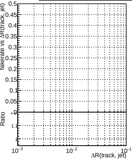
Fake rate vs \Delta R(\text{track, jet}) DQM_TT_original DQM_TT_newscoreonlyINT
