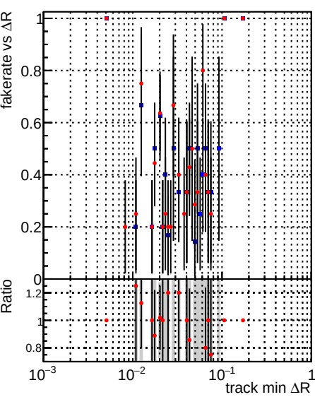
Fake rate vs \Delta R(\text{track, jet}) DQM_TT_original DQM_TT_newscoreonlyINT
