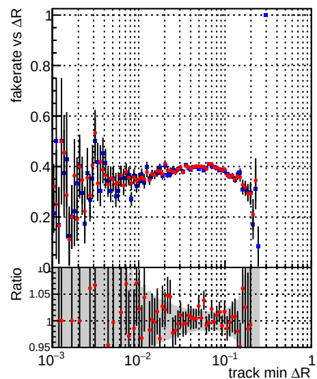
—■— DQM_TT_original —●— DQM_TT_newscoreonlyINT
