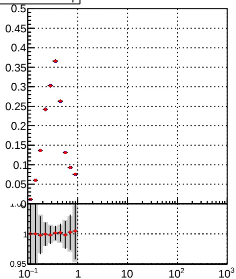
DQM_TT_mkFit-DQM_original DQM_TT_mkFit-DQM_modified5
