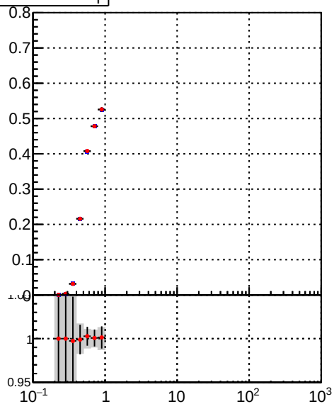
— DQM_TT_mkFit-DQM_original — DQM_TT_mkFit-DQM_modified5
