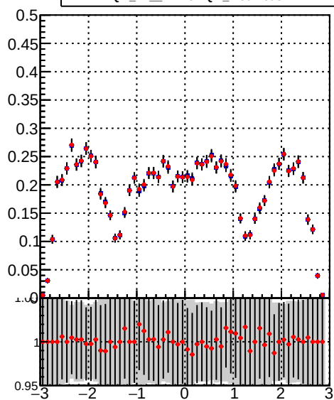
— DQM_TT_mkFit-DQM_original — DQM_TT_mkFit-DQM_modified5
