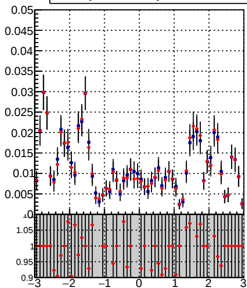
DQM_TT_mkFit-DQM_original DQM_TT_mkFit-DQM_modified5
