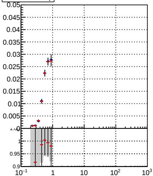
DQM_TT_mkFit-DQM_original DQM_TT_mkFit-DQM_modified5
